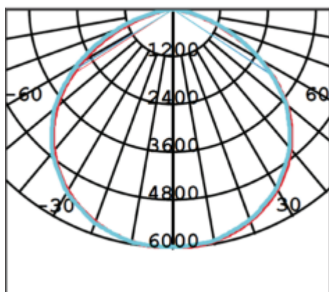
PHOTOMETRIC DIAGRAM
